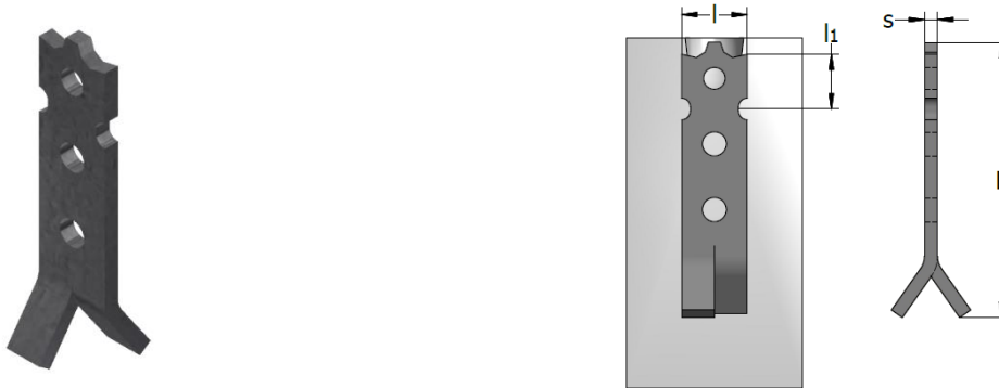
UNIVERSAL ANCHOR 12.5 kN, DIMENSIONS AND LOAD CAPACITY
